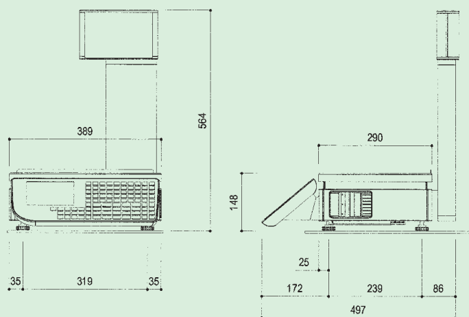
equa 3000LOOK T TORRETTA
